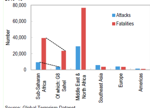
Figure 1.1.2. Selected Regions: Regional Distribution of Terrorism, 2010–16
